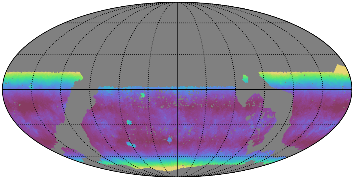
mw_roll_bulge_v3.3_10yrs WFD z band: Median airmass
