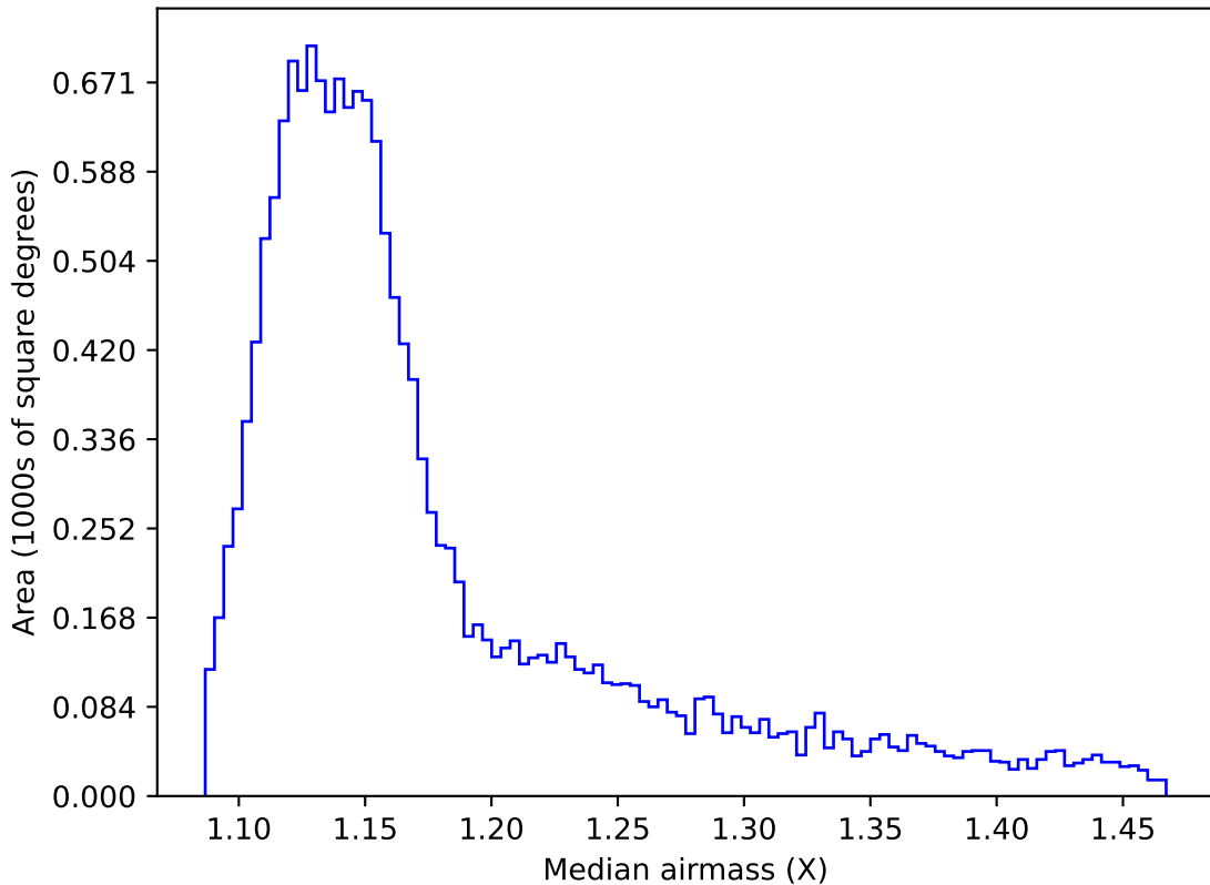
mw_roll_bulge_v3.3_10yrs WFD z band: Median airmass
