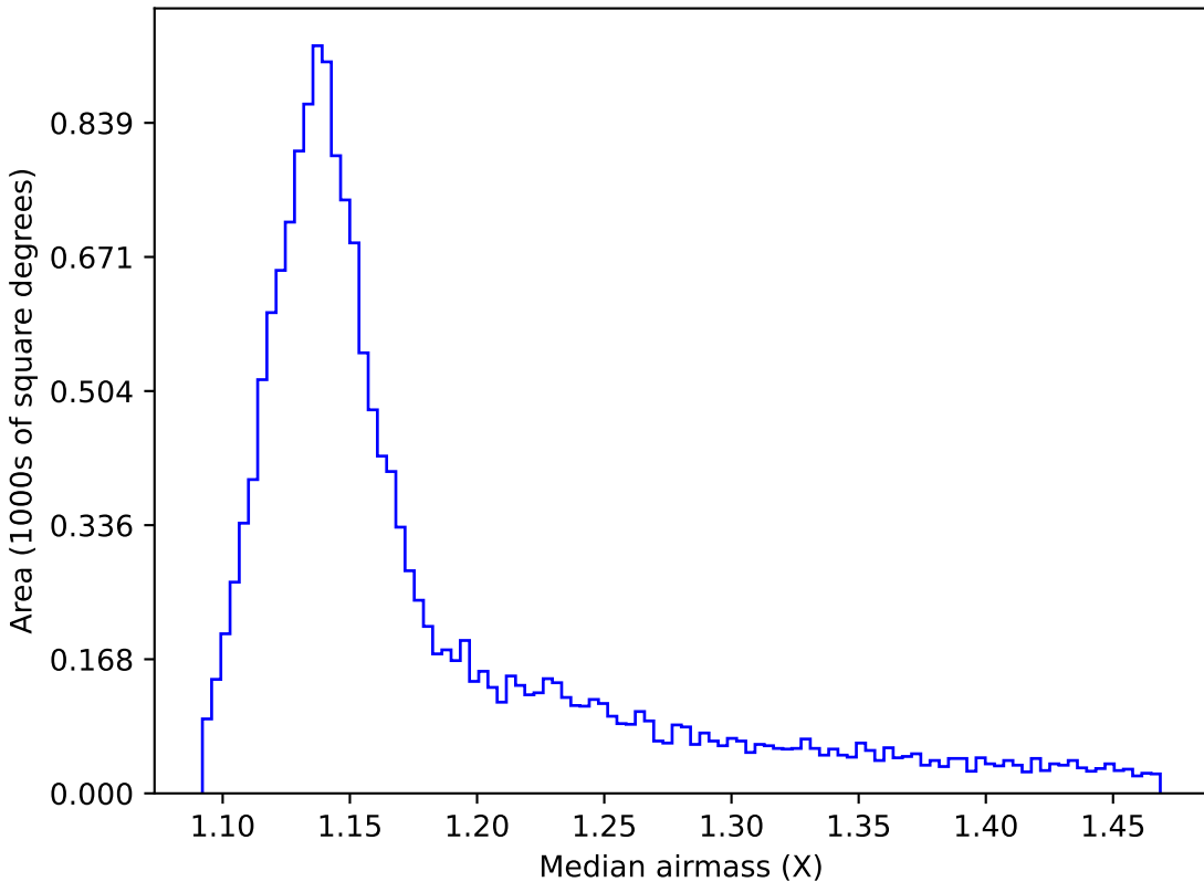
mw_roll_bulge_v3.3_10yrs WFD y band: Median airmass
