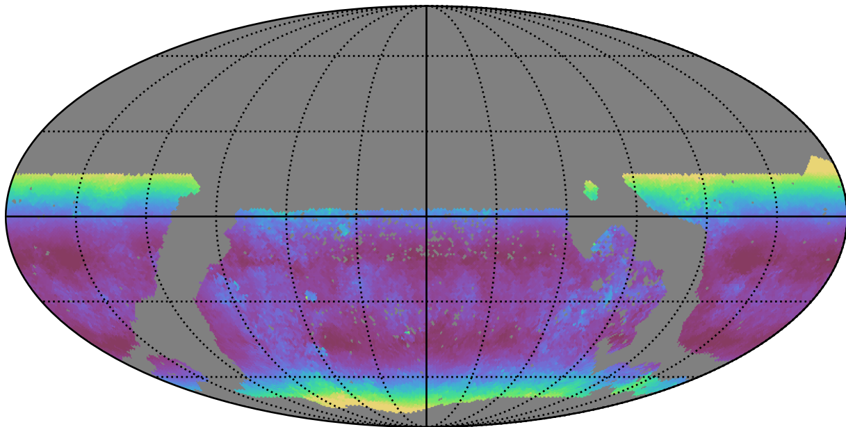
mw_roll_bulge_v3.3_10yrs WFD u band: Median airmass
