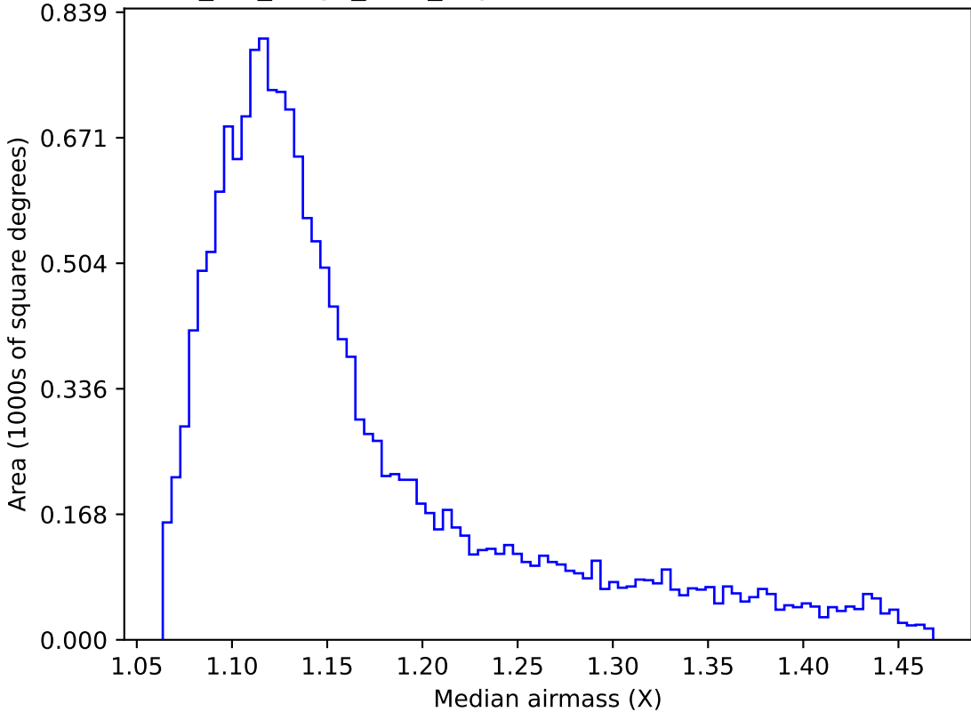
mw_roll_bulge_v3.3_10yrs WFD u band: Median airmass
