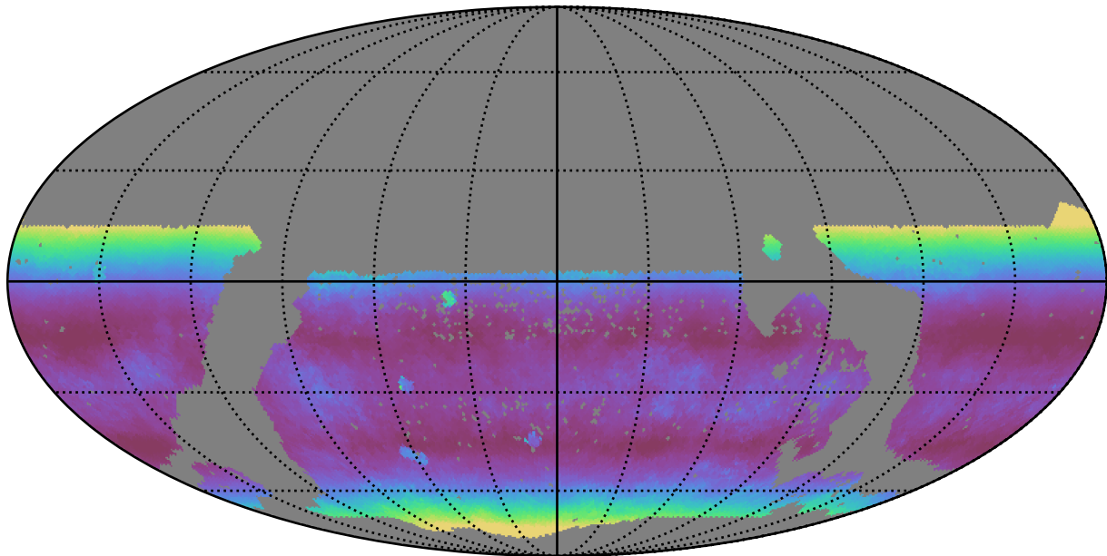
mw_roll_bulge_v3.3_10yrs WFD r band: Median airmass
