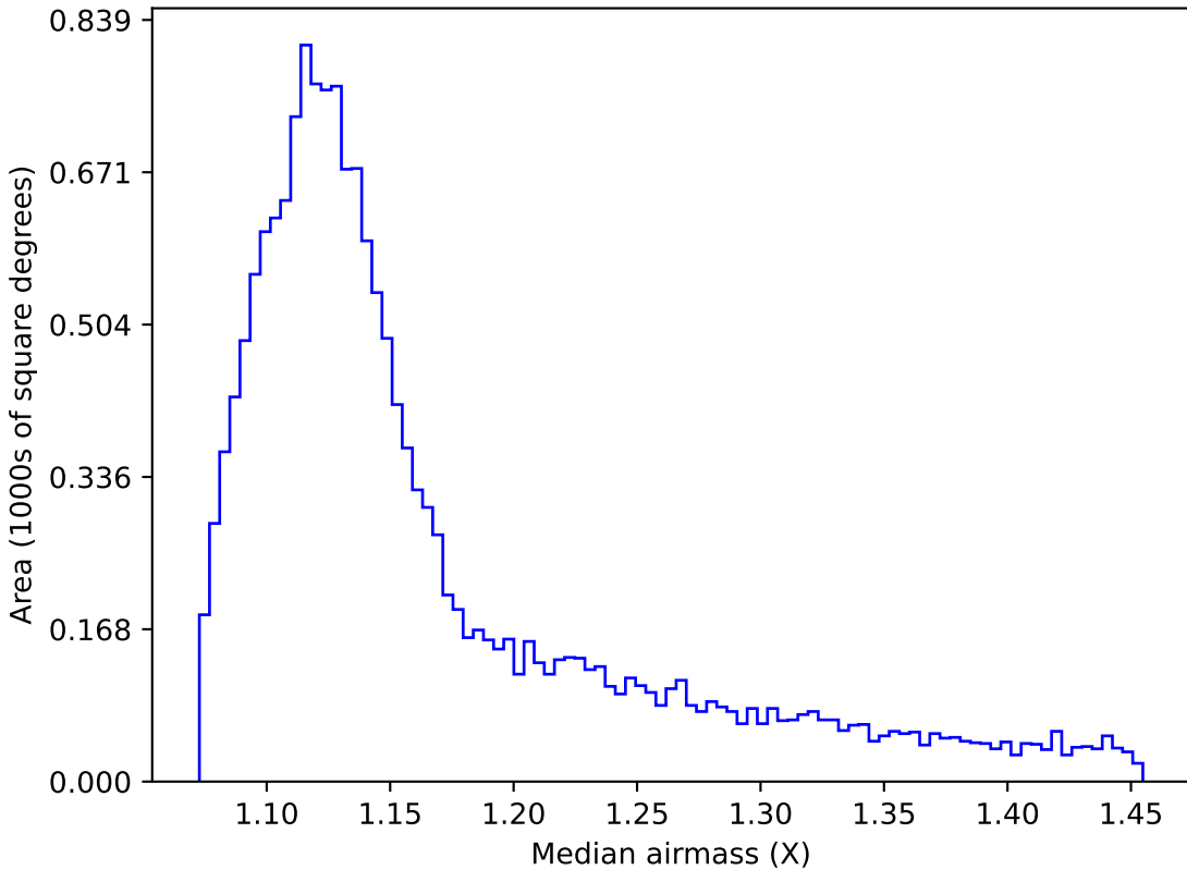
mw_roll_bulge_v3.3_10yrs WFD r band: Median airmass
