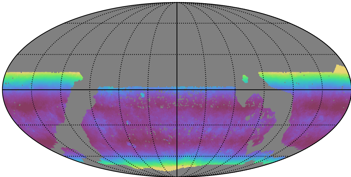
mw_roll_bulge_v3.3_10yrs WFD i band: Median airmass
