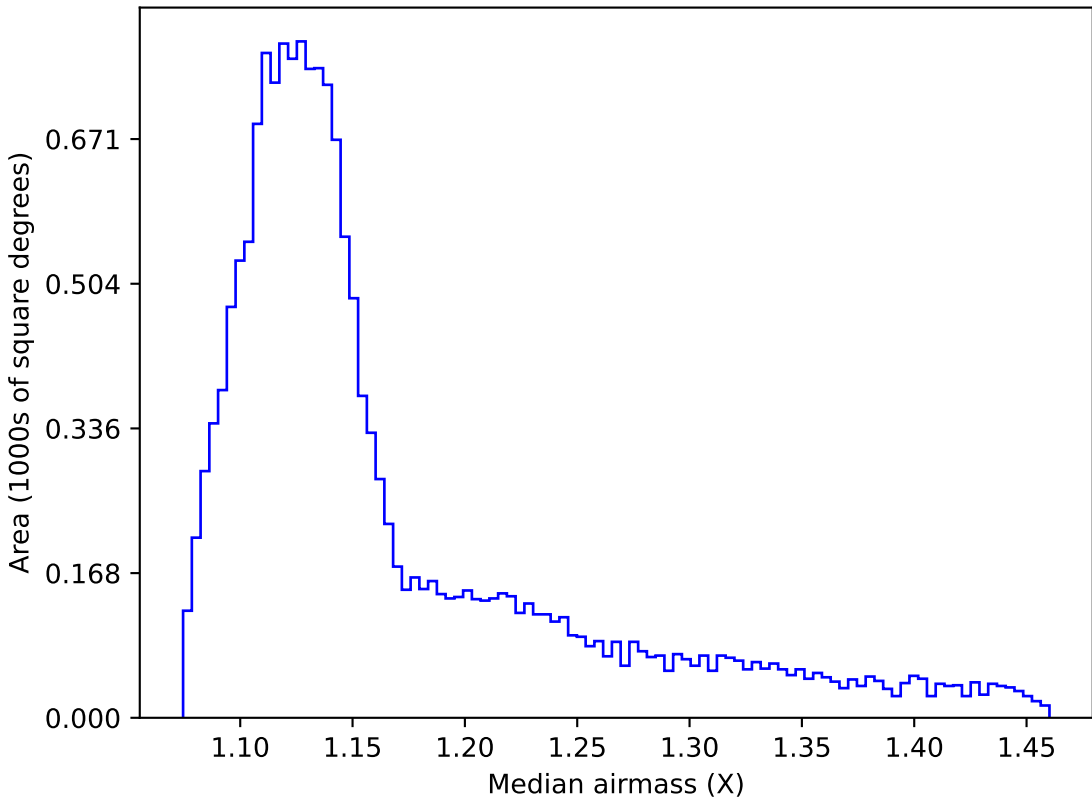
mw_roll_bulge_v3.3_10yrs WFD i band: Median airmass
