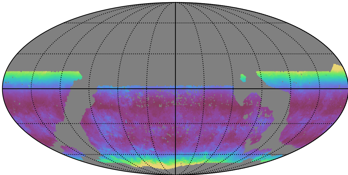
mw_roll_bulge_v3.3_10yrs WFD g band: Median airmass
