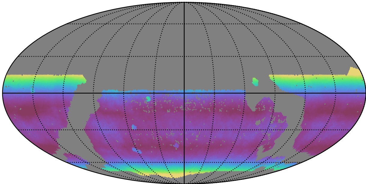
mw_roll_bulge_v3.3_10yrs WFD all bands: Median airmass
