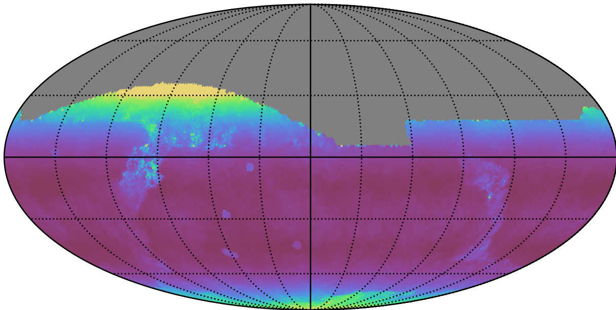
mw_roll_bulge_v3.3_10yrs All sky z band: Median airmass
