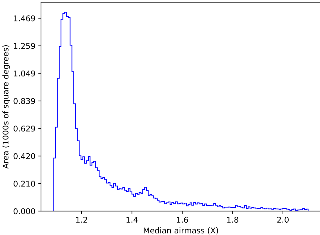
mw_roll_bulge_v3.3_10yrs All sky z band: Median airmass
