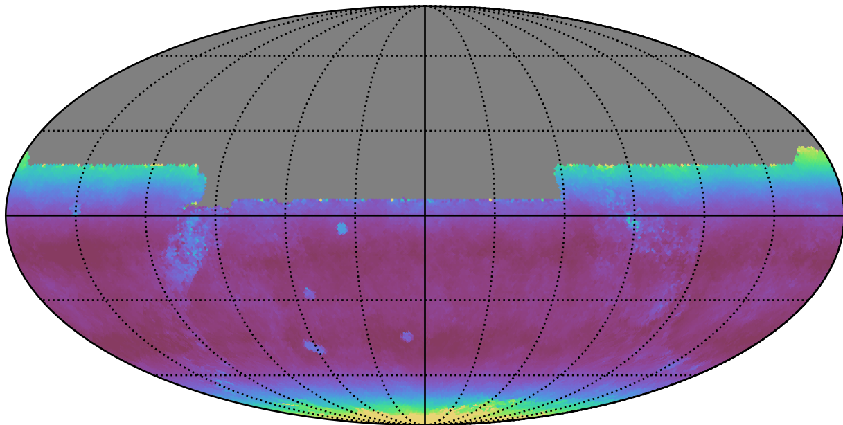
mw_roll_bulge_v3.3_10yrs All sky y band: Median airmass
