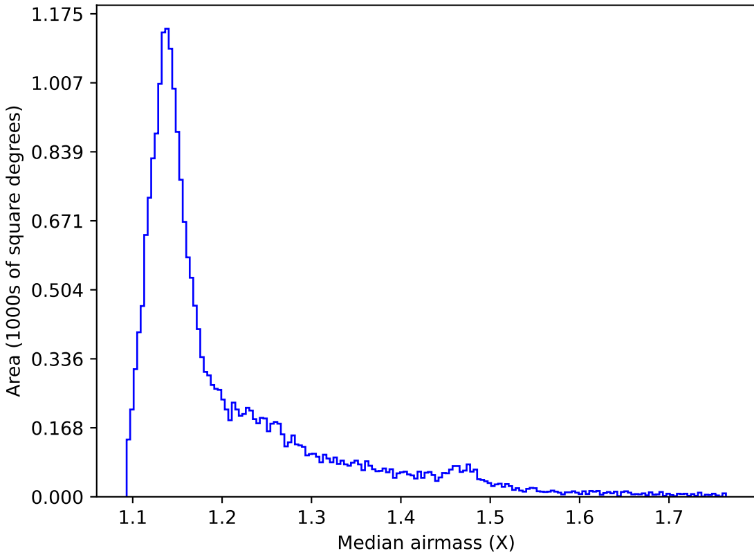
mw_roll_bulge_v3.3_10yrs All sky y band: Median airmass
