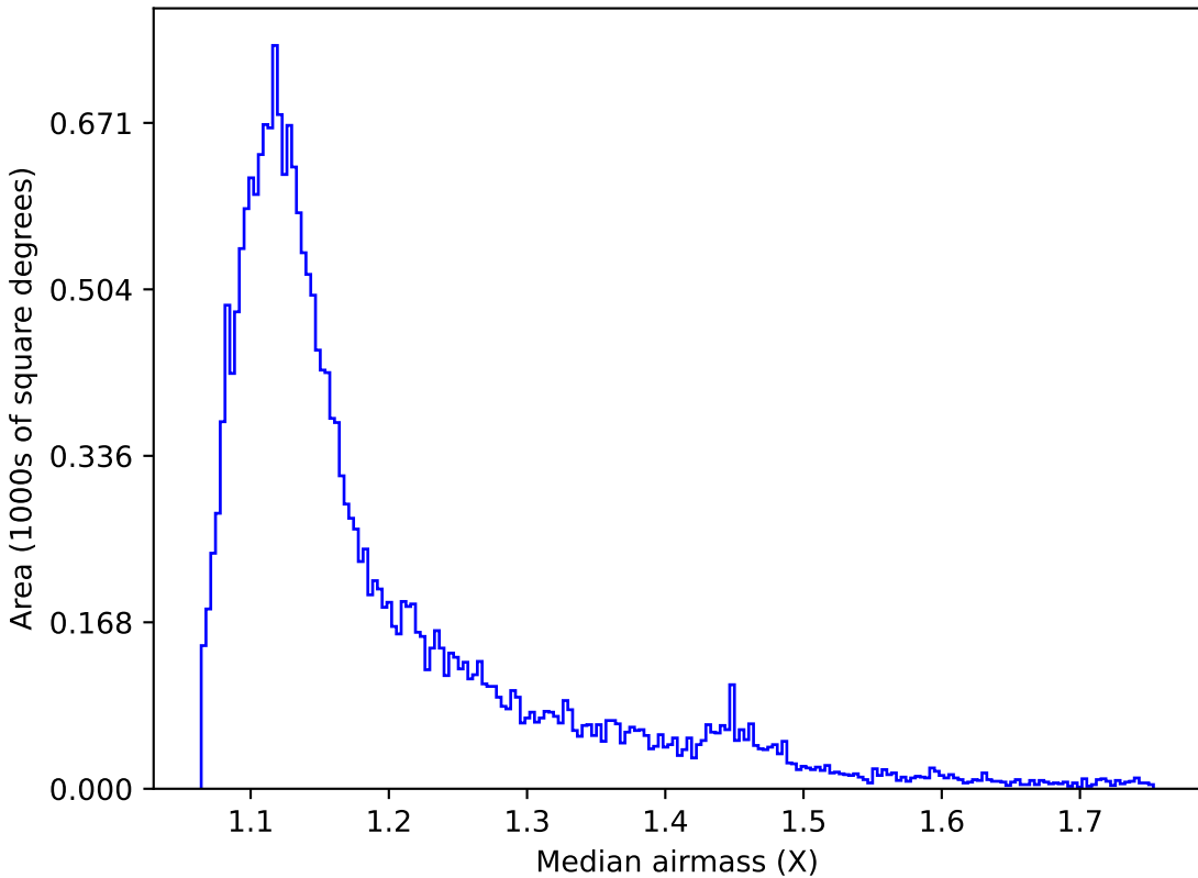
mw_roll_bulge_v3.3_10yrs All sky u band: Median airmass
