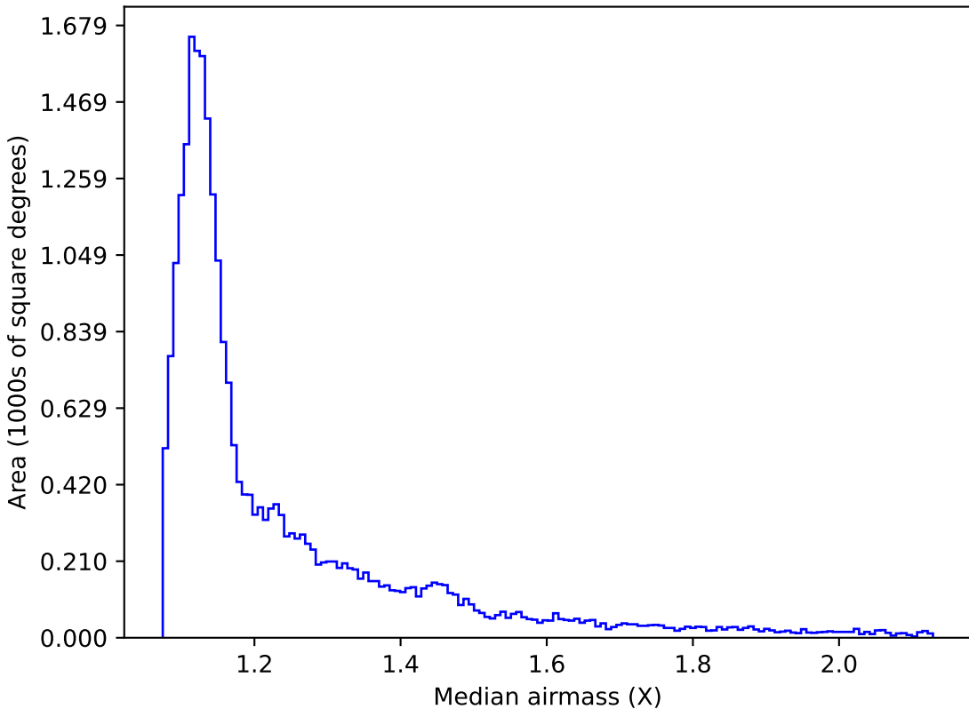
mw_roll_bulge_v3.3_10yrs All sky r band: Median airmass
