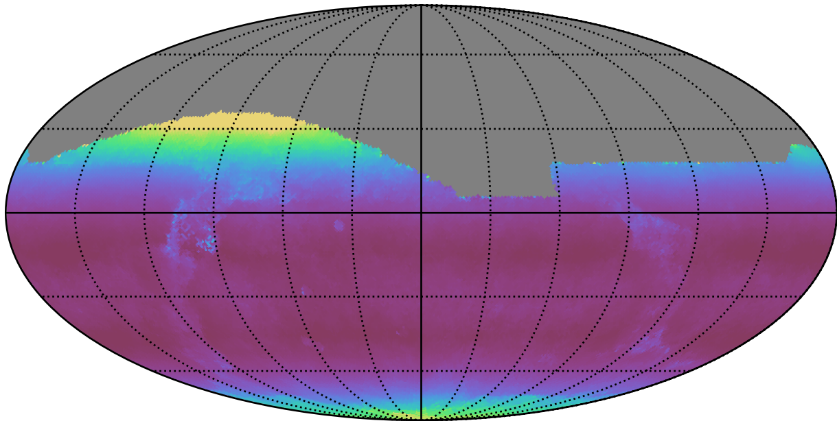
mw_roll_bulge_v3.3_10yrs All sky i band: Median airmass
