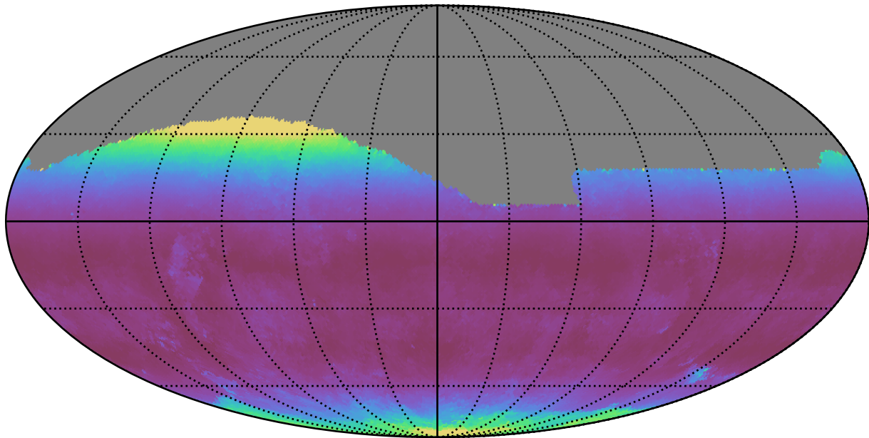
mw_roll_bulge_v3.3_10yrs All sky g band: Median airmass
