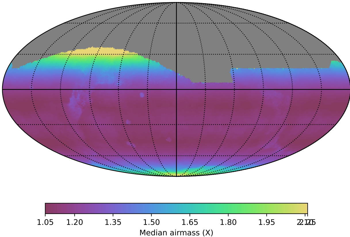
mw_roll_bulge_v3.3_10yrs All sky all bands: Median airmass
