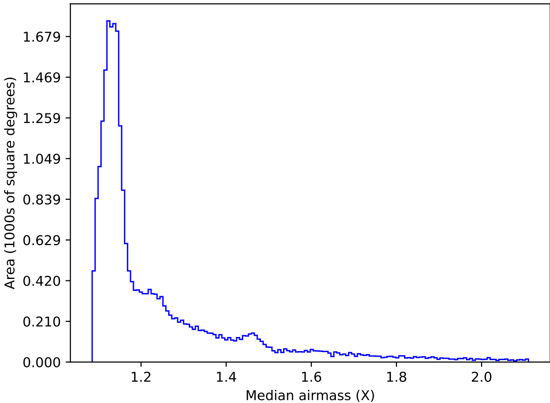
mw_roll_bulge_v3.3_10yrs All sky all bands: Median airmass
