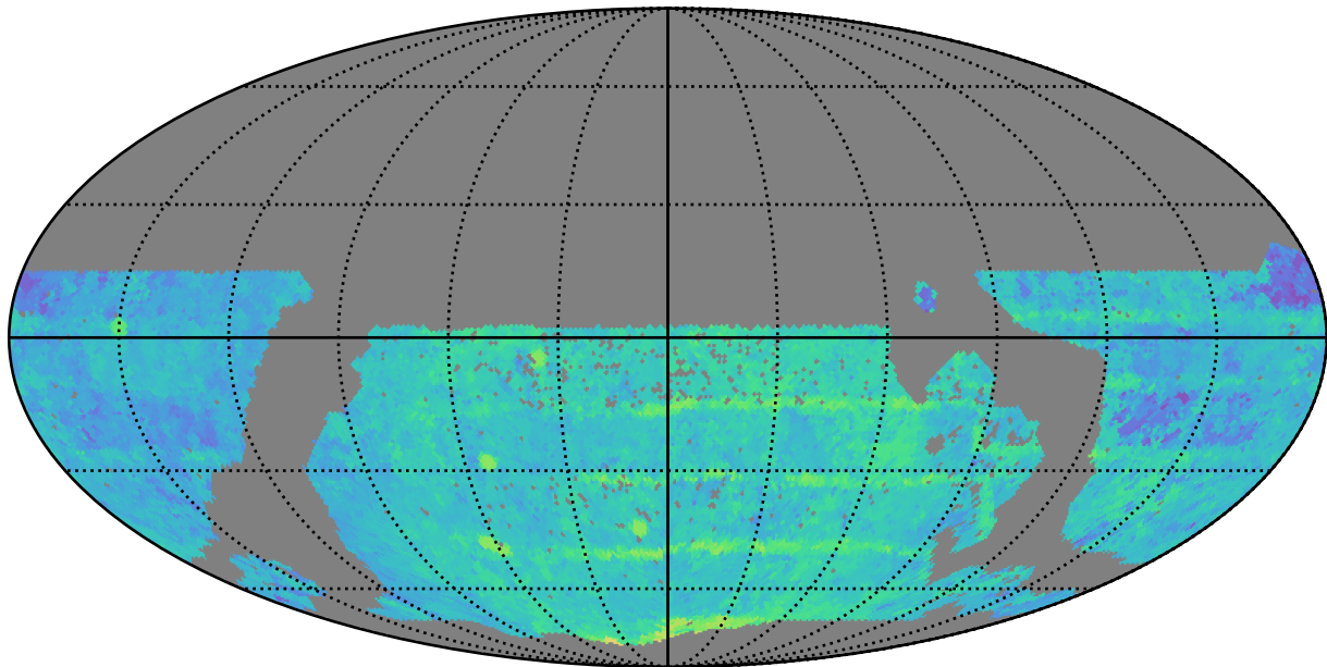
mw_roll_bulge_v3.3_10yrs WFD z band: Median Season Length
