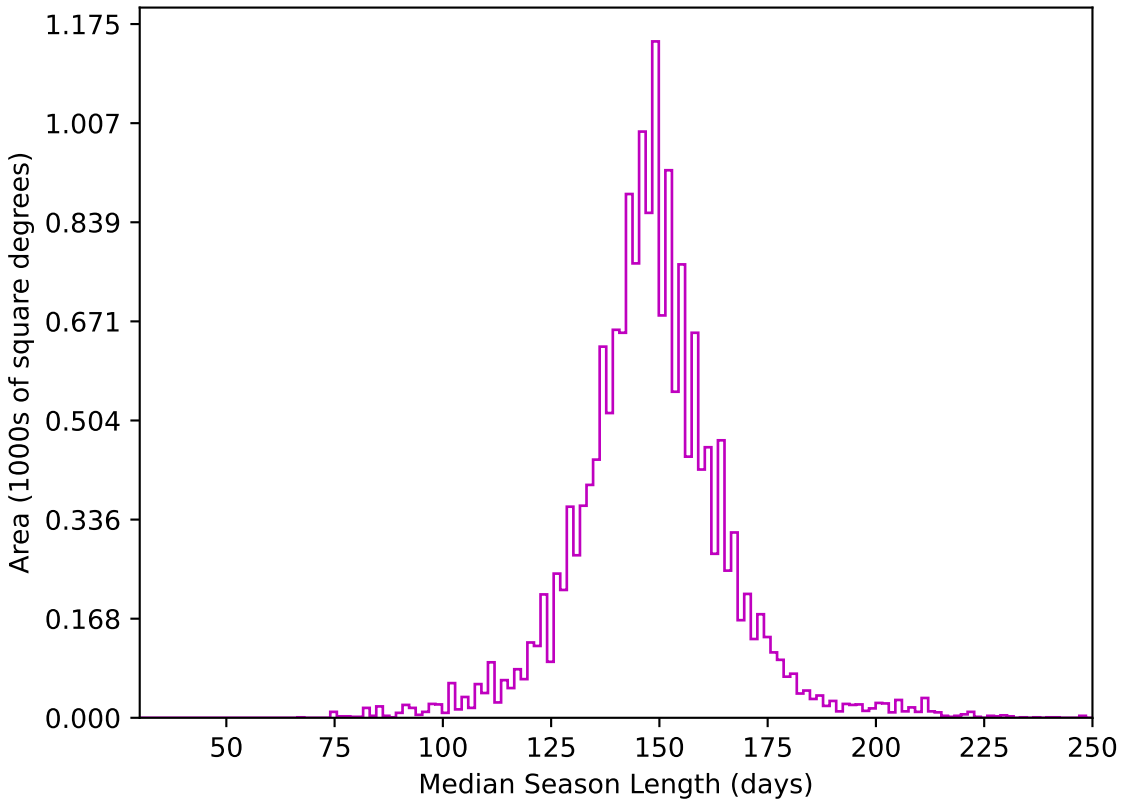
mw_roll_bulge_v3.3_10yrs WFD z band: Median Season Length
