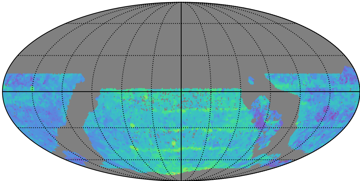
mw_roll_bulge_v3.3_10yrs WFD y band: Median Season Length
