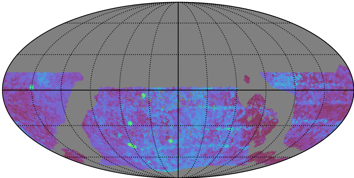
mw_roll_bulge_v3.3_10yrs WFD u band: Median Season Length
