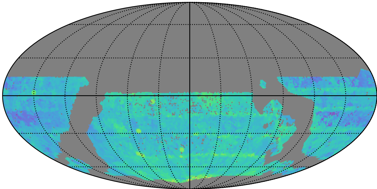
mw_roll_bulge_v3.3_10yrs WFD i band: Median Season Length
