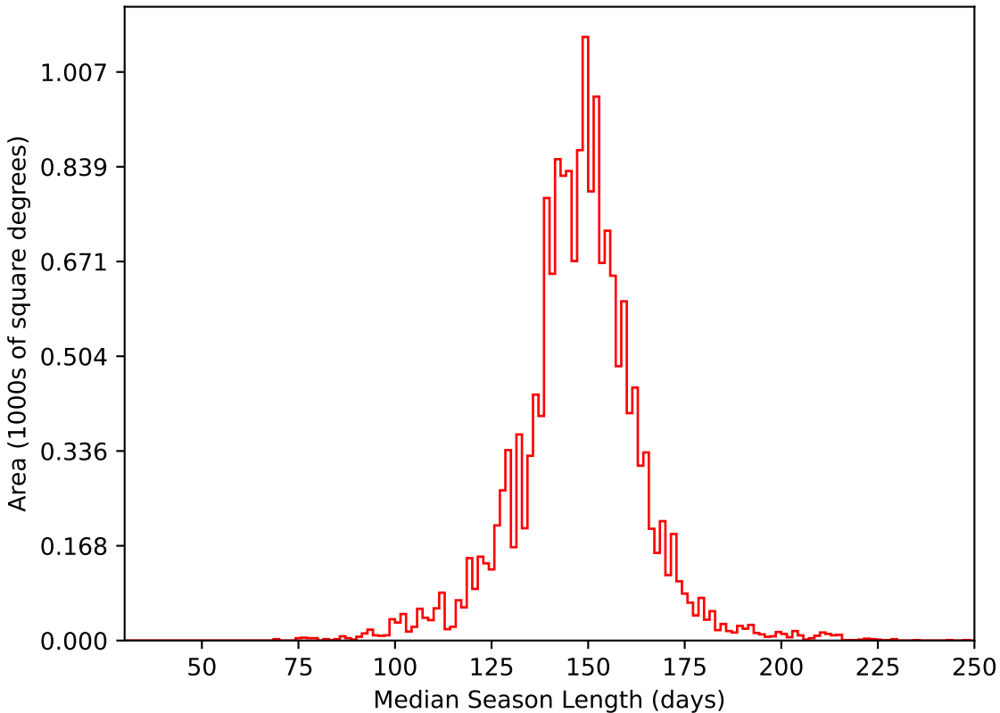
mw_roll_bulge_v3.3_10yrs WFD i band: Median Season Length
