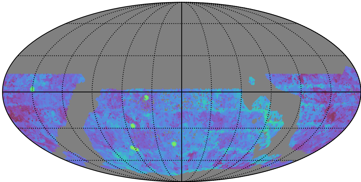
mw_roll_bulge_v3.3_10yrs WFD g band: Median Season Length
