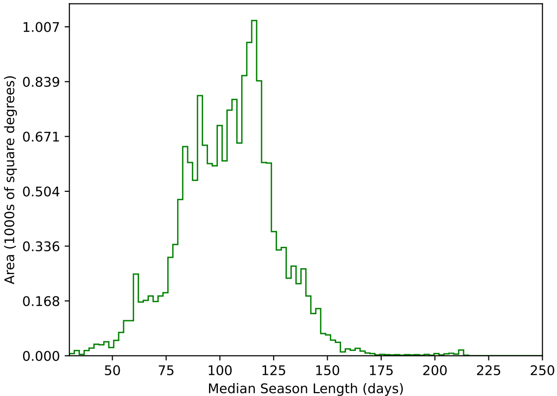
mw_roll_bulge_v3.3_10yrs WFD g band: Median Season Length
