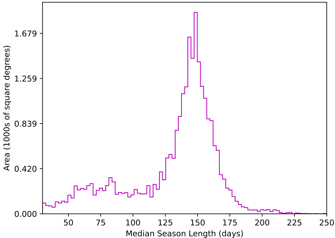
mw_roll_bulge_v3.3_10yrs All sky z band: Median Season Length
