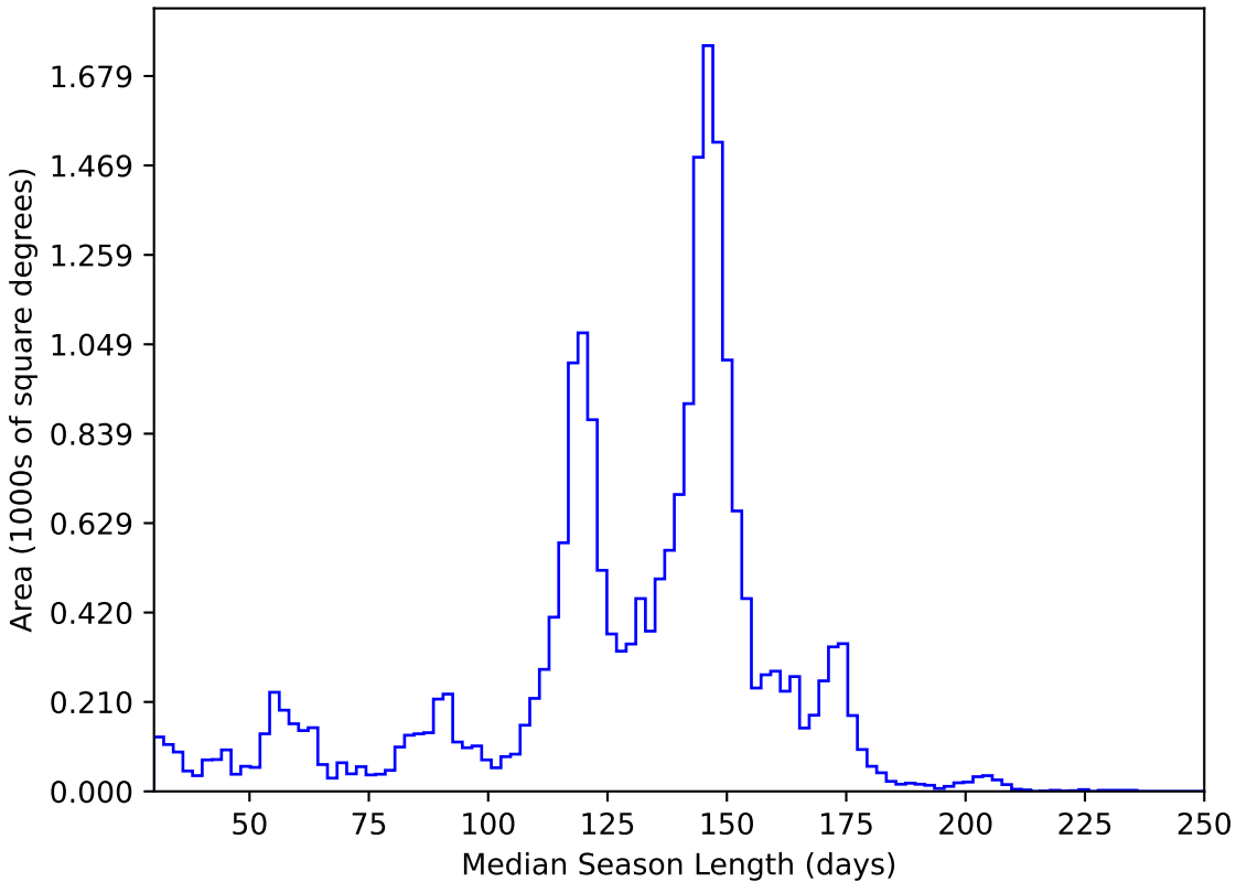
mw_roll_bulge_v3.3_10yrs All sky y band: Median Season Length
