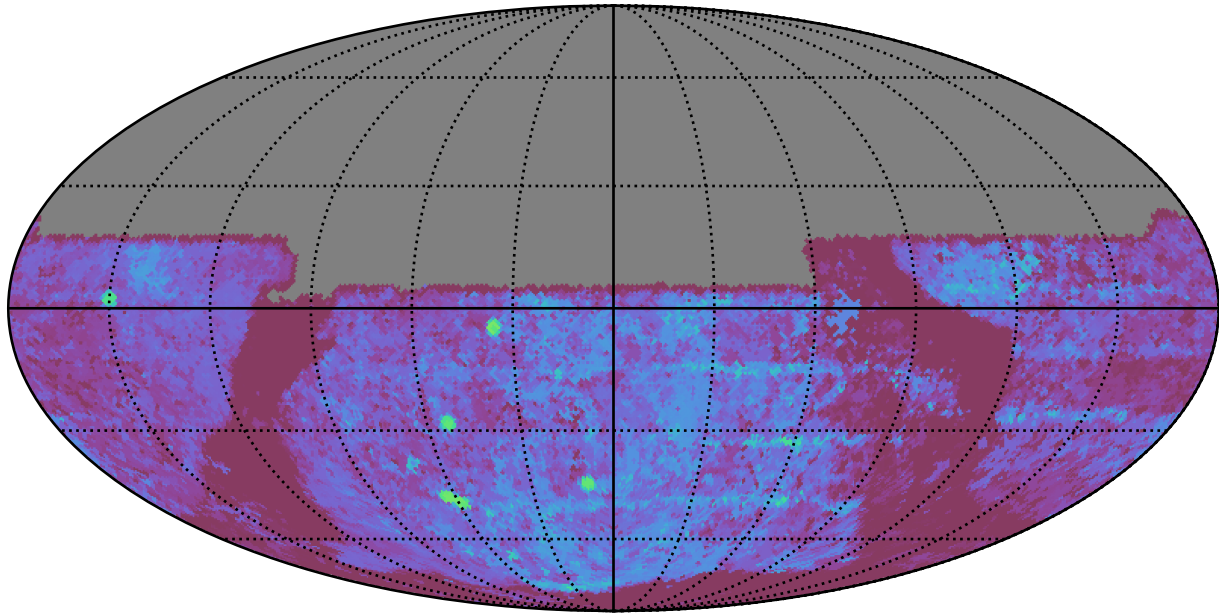
mw_roll_bulge_v3.3_10yrs All sky u band: Median Season Length
