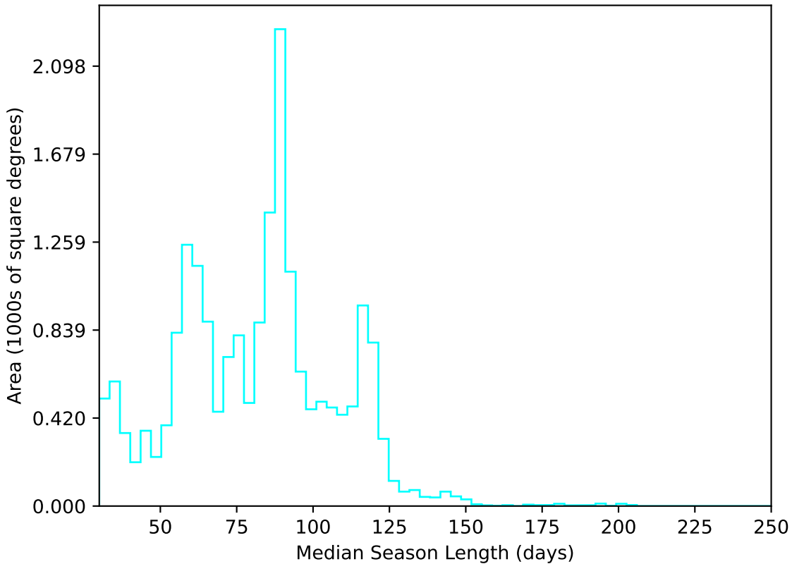
mw_roll_bulge_v3.3_10yrs All sky u band: Median Season Length
