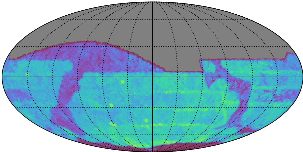
mw_roll_bulge_v3.3_10yrs All sky r band: Median Season Length
