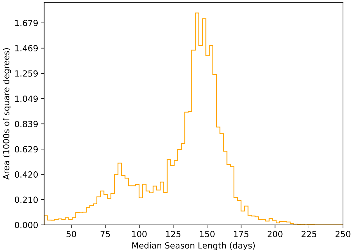
mw_roll_bulge_v3.3_10yrs All sky r band: Median Season Length
