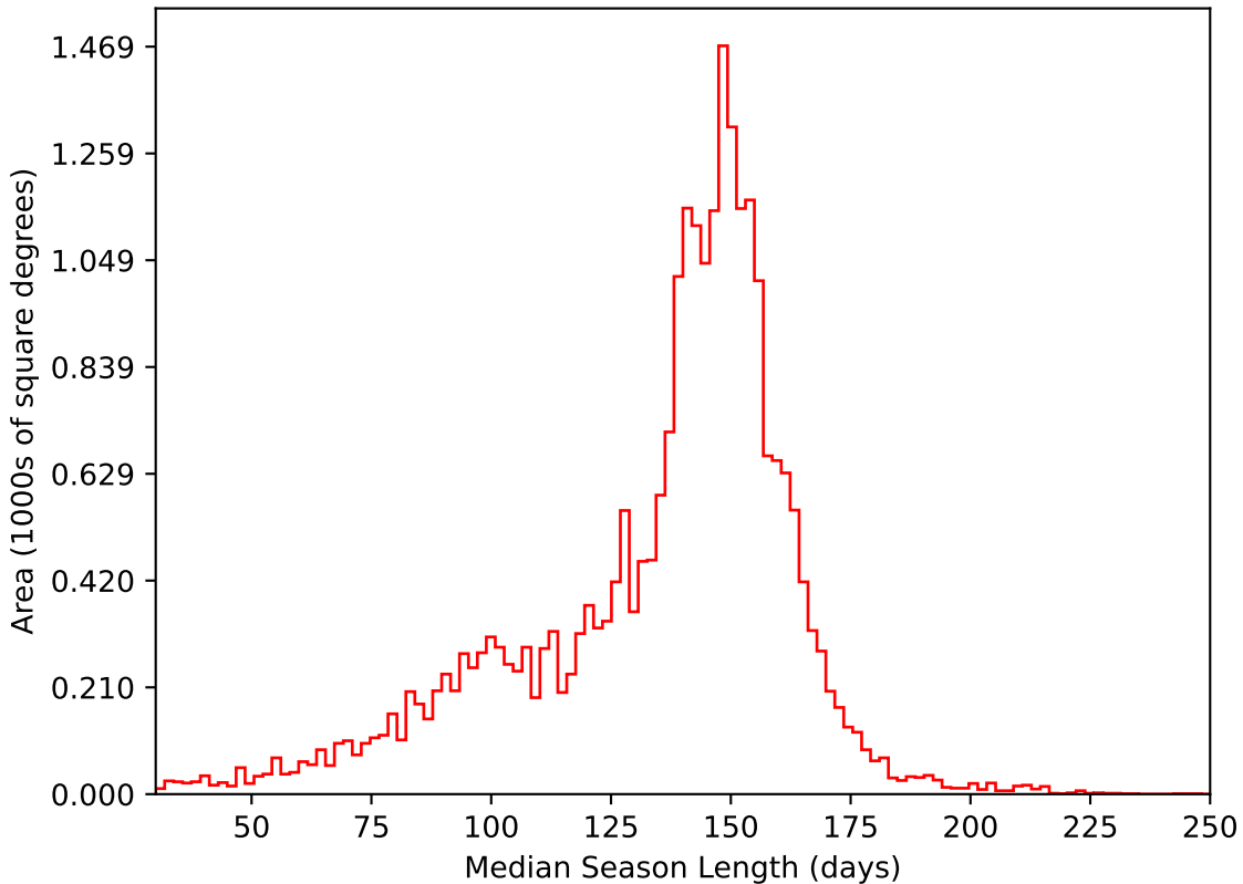
mw_roll_bulge_v3.3_10yrs All sky i band: Median Season Length
