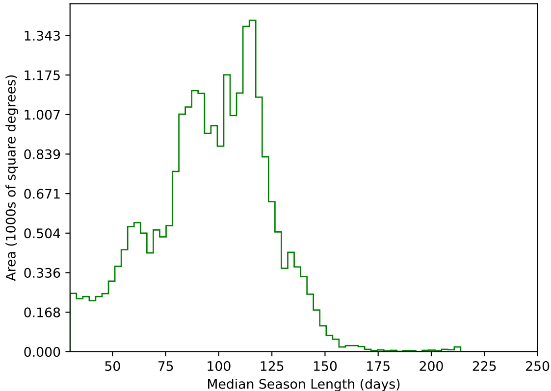
mw_roll_bulge_v3.3_10yrs All sky g band: Median Season Length
