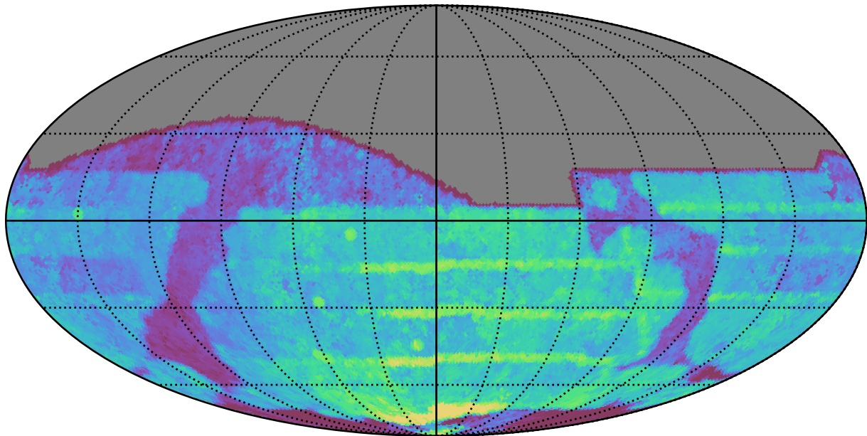
mw_roll_bulge_v3.3_10yrs All sky all bands: Median Season Length
