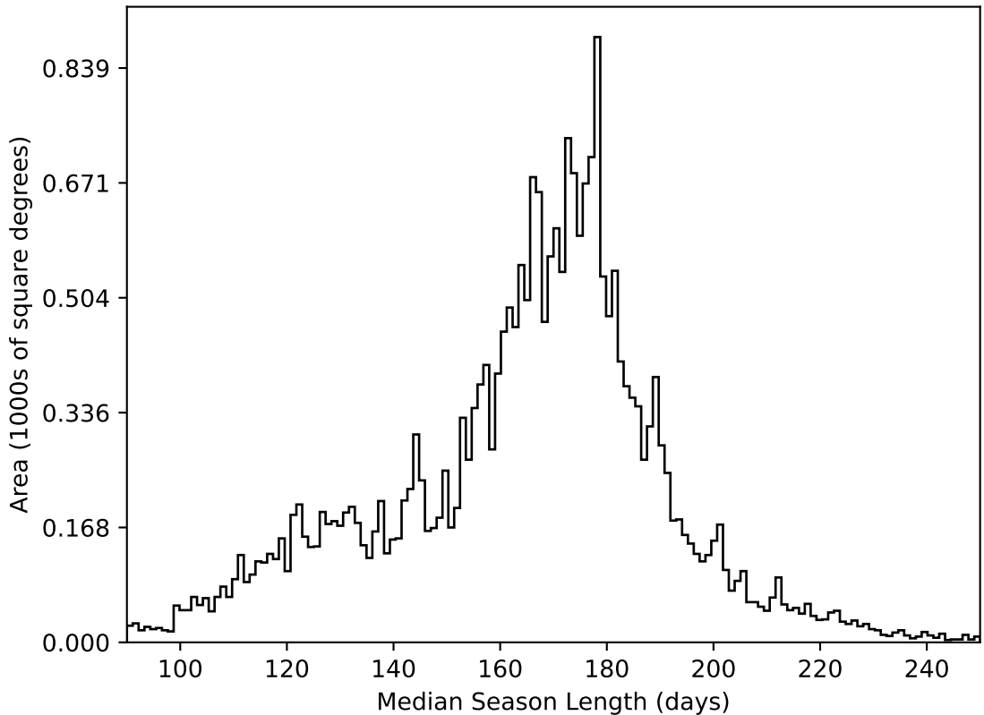
mw_roll_bulge_v3.3_10yrs All sky all bands: Median Season Length
