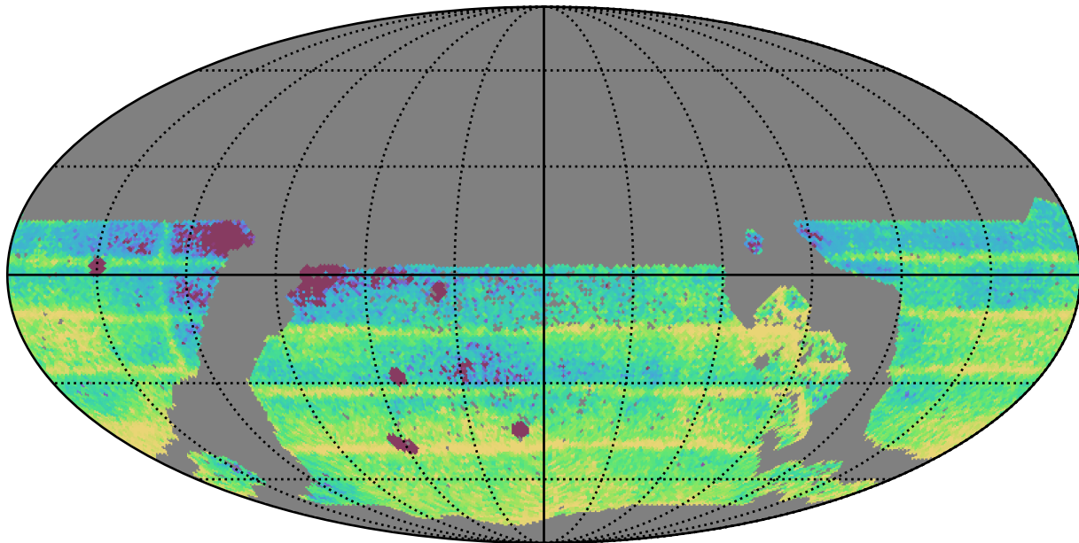
mw_roll_bulge_v3.3_10yrs WFD: Median Intra-Night Gap
