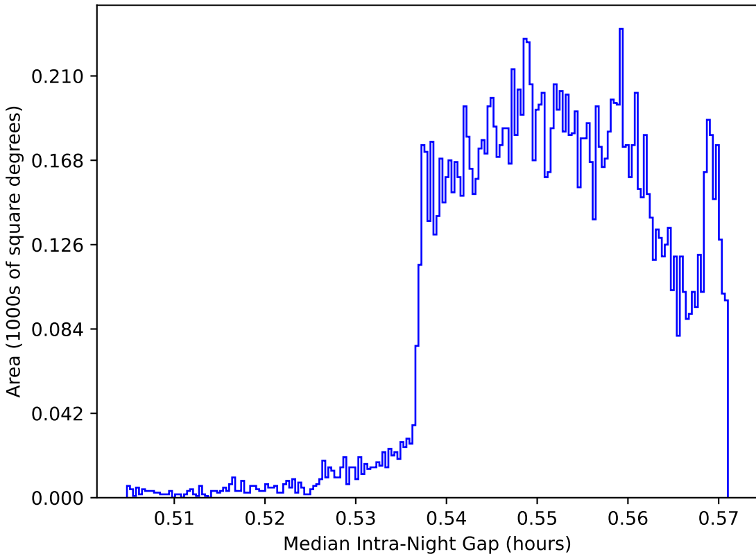
mw_roll_bulge_v3.3_10yrs WFD: Median Intra-Night Gap
