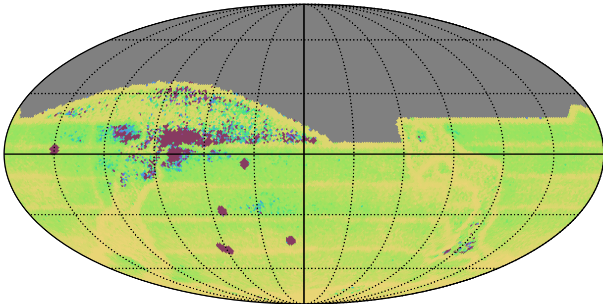
mw_roll_bulge_v3.3_10yrs All sky: Median Intra-Night Gap
