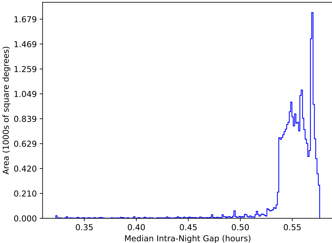
mw_roll_bulge_v3.3_10yrs All sky: Median Intra-Night Gap
