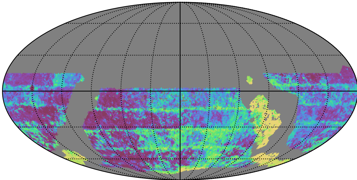
mw_roll_bulge_v3.3_10yrs WFD y band: Median Inter-Night Gap
