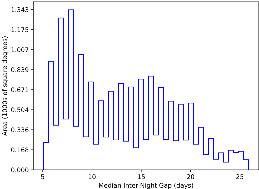
mw_roll_bulge_v3.3_10yrs WFD y band: Median Inter-Night Gap
