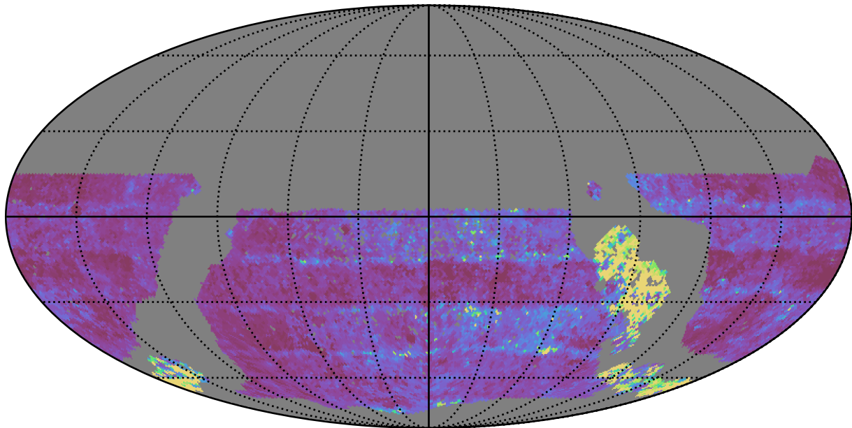
mw_roll_bulge_v3.3_10yrs WFD u band: Median Inter-Night Gap
