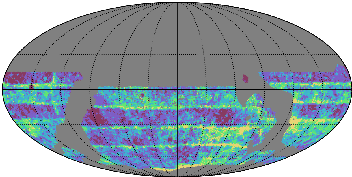
mw_roll_bulge_v3.3_10yrs WFD i band: Median Inter-Night Gap
