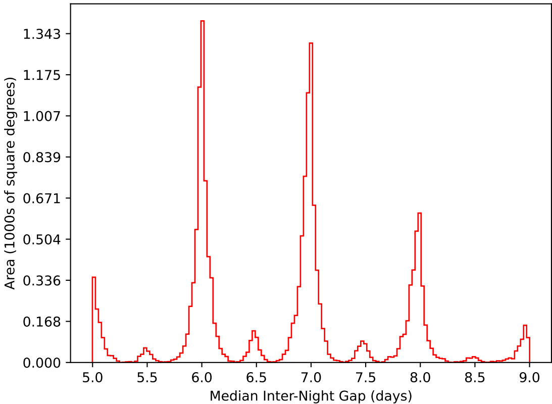
mw_roll_bulge_v3.3_10yrs WFD i band: Median Inter-Night Gap
