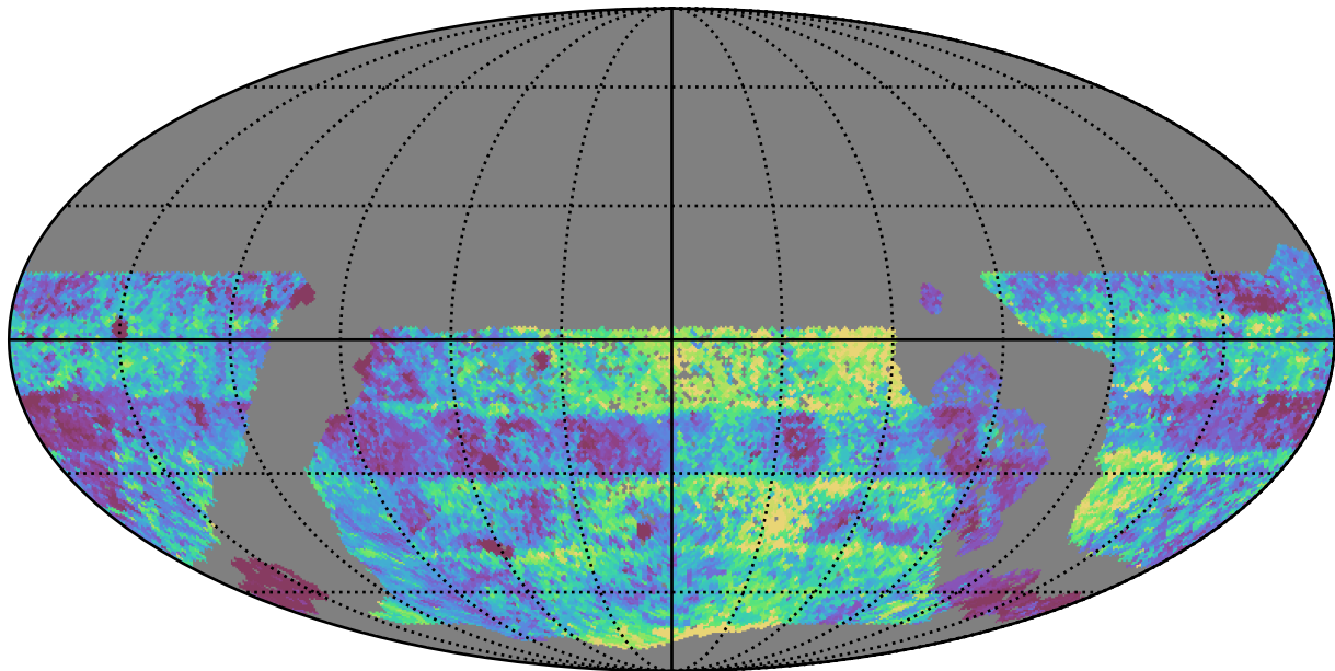
mw_roll_bulge_v3.3_10yrs WFD g band: Median Inter-Night Gap
