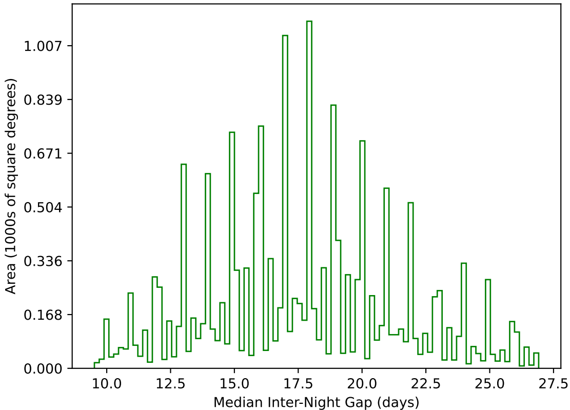
mw_roll_bulge_v3.3_10yrs WFD g band: Median Inter-Night Gap
